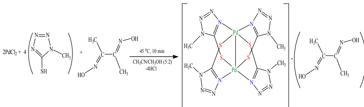
Scheme 3. The preparation method for complex 1
